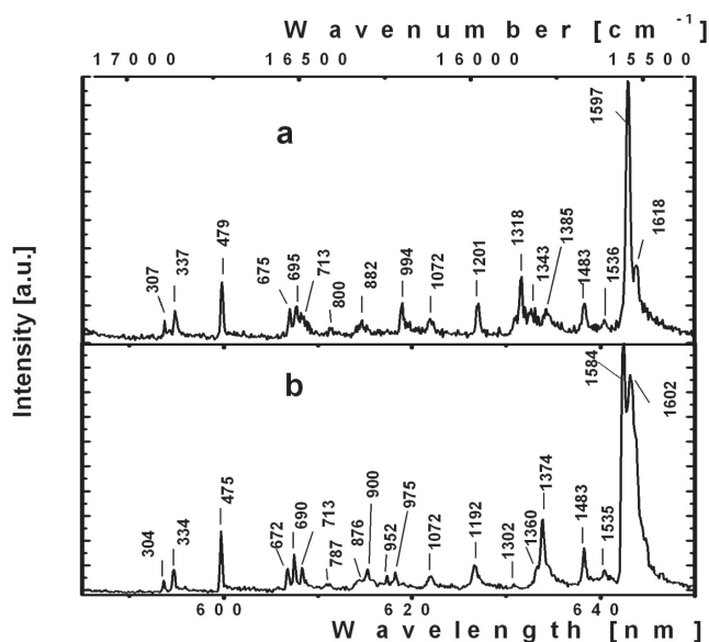
Figure 3. FLN spectra of H_4P^{2+} in the mixture of acetonitrile/ 10^{-3}M HClO_4 (a) and D_4P^{2+} in the mixture of acetonitrile/ 10^{-3}M D_2SO_4 (b) upon selective excitation ( \lambda_{exc}=585 nm) at 4.2 K.
